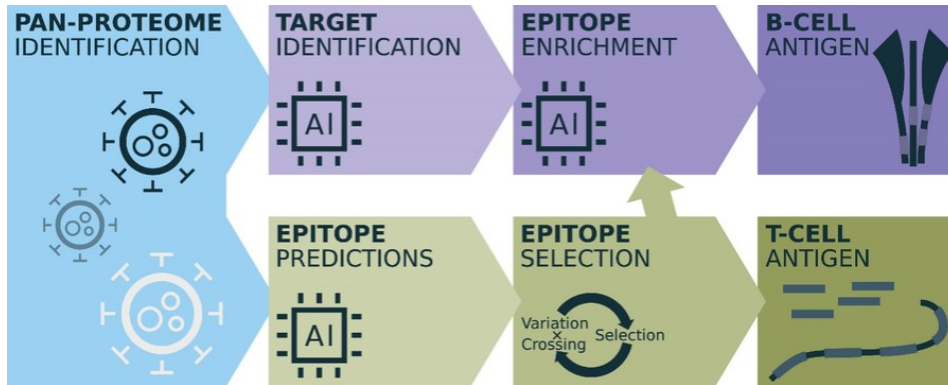
Figure 37: RAVEN workflow.
