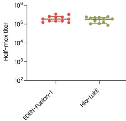
Figure 42: IgG titers. Mice were immunized with EVX-B1. IgG titers are shown as half-max titers for individual mice, groups median values and 95% confidence interwall are shown.
