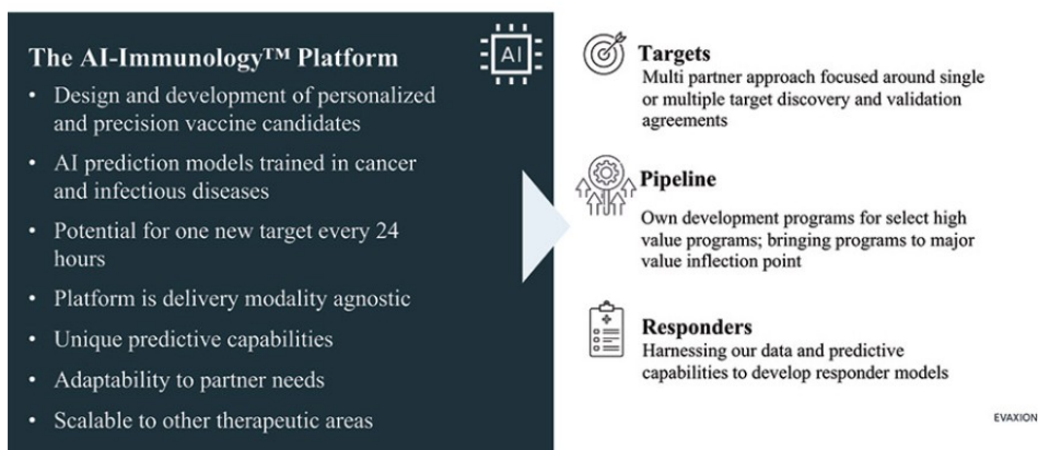
Figure 6: The Evaxion Strategy.
