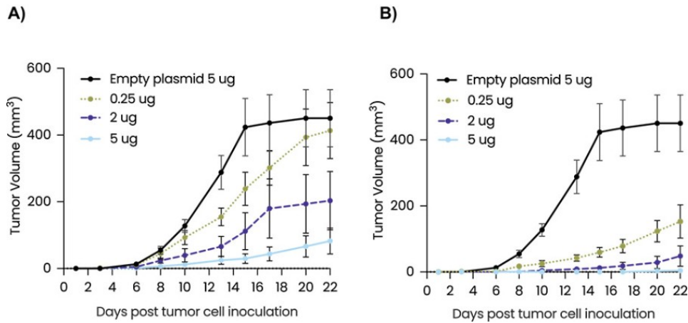
Figure 30: mEVX-02 A) and mEVX-03 B) dose-dependently inhibited the growth of subcutaneous CT26 tumors. Antitumor of EVX-02 and EVX-03 was obtained at doses as low as 5 and 0.25 \mu\text{g} , respectively.
