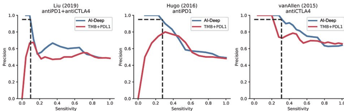
Figure 34: Prediction of patient response to immunotherapy from genomic profiles, neoantigen and ERV antigen signatures in baseline tumor biopsy. Genomic data of baseline biopsies from 937 CPI treated cancer patients were curated from 14 studies and divided in 3 cohorts. AI-DeeP™ (blue line) predicts a subset of progressive disease patients with high precision. In the anti-PD1 & anti-CTLA4 treated cohort, AI-DeeP™ can identify 10% of the non-responding patients with 95% precision, versus with classical biomarkers (‘TMB & PD-L1’, red line) with 70% precision. In the anti-PD1 treated cohort, AI-DeeP™ can identify 25% of the non-responding patients with 95% precision, versus with classical biomarkers with 80% precision. In the anti-CTLA4 treated cohort, AI-DeeP™ can identify 30% of the non-responding patients with 95% precision, versus with classical biomarkers with 70% precision.
