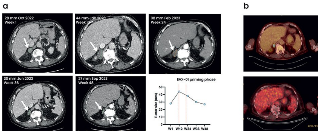
Figure 25: Longitudinal reduction in tumor volume for patient 100004. a) the tumor size was 28 mm at baseline (Oct 2022). Prior to EVX-01 administration and following 12 weeks of pembrolizumab, the patient presented with Progressive Disease (RECIST1.1 criteria), tumor size 44 mm (Jan 2023). Following EVX-01 administration, the patient started to respond to treatment showing a reduction in tumor size at week 24 (38 mm). This was further confirmed at the assessments week 36 (Jun 2023) and 48 (Sep 2023) where the target lesion was 30 mm and 27 mm, respectively. b) Patient 100004 FDG PET scan demonstrating complete metabolic response at week 52 with resolution of FDG avidity in the right adrenal target lesion.
