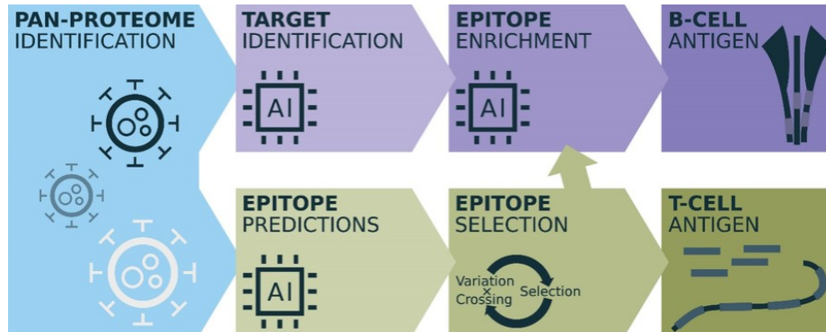
Figure 37: RAVEN workflow.
